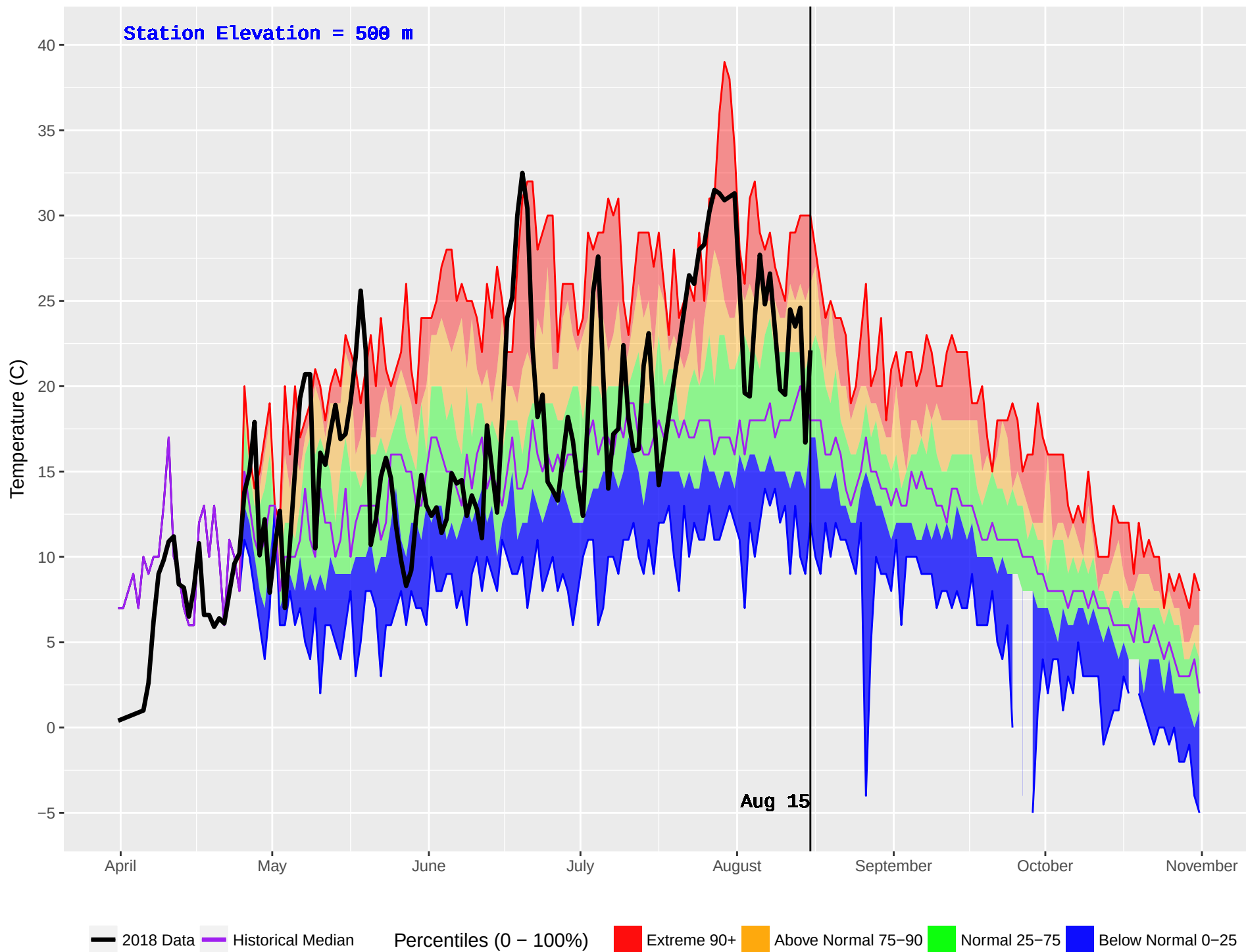
CRANBERRY (433) : Historical (1995–2016) and Current (2018) Daily Temperature
